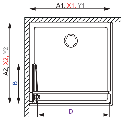
Wariant LEWY Variant L
